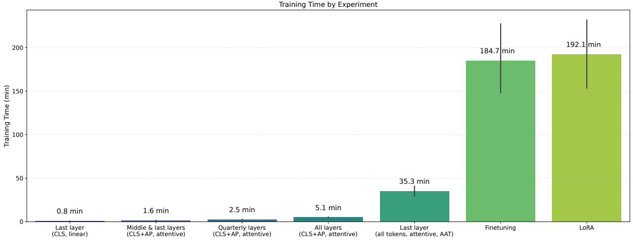
Figure 19. Training times in minutes for probing strategies and finetuning averaged across datasets and the three base models.
